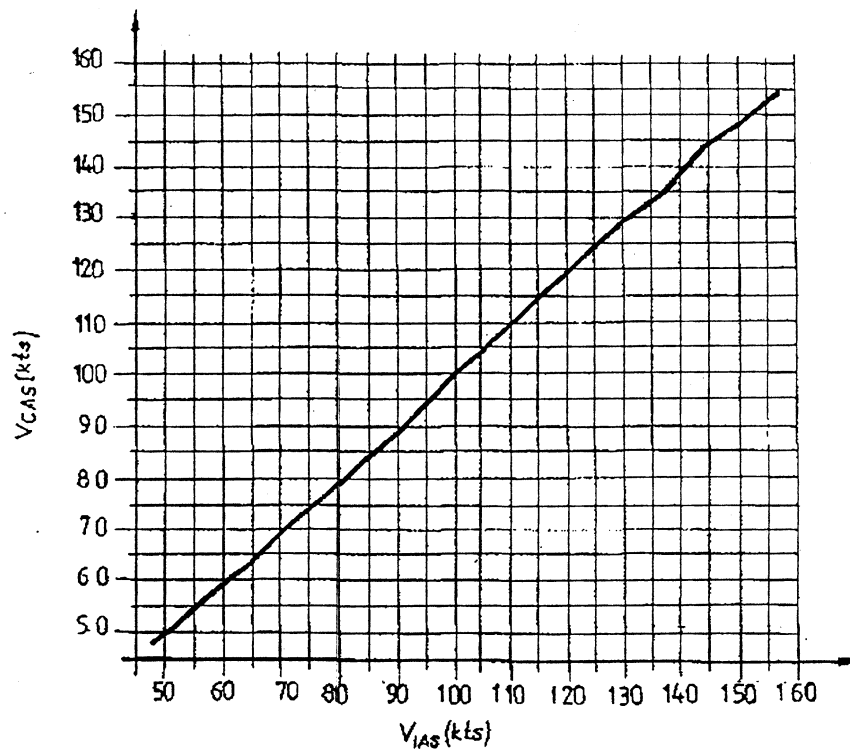
Airspeed Indicator System Calibration
