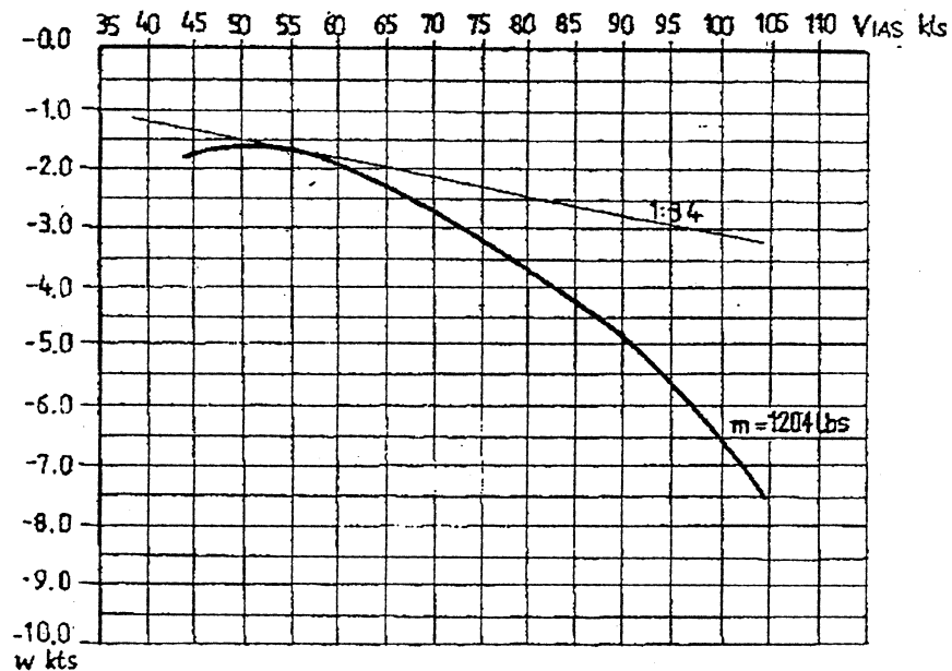
Flight Polar Fig. 5-2
